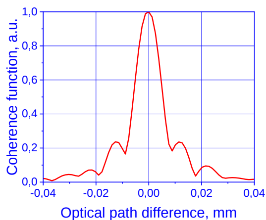
Coherence function at 15 mW SMF
