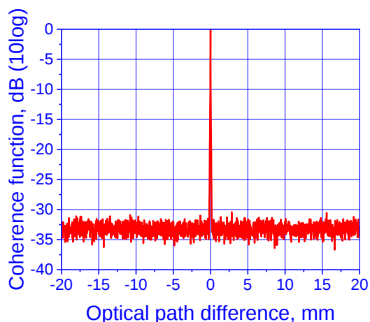
Coherence at 15 mW output (extended plot)
