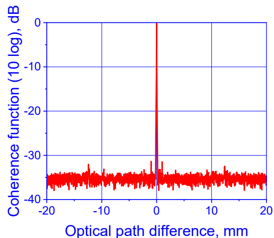
Coherence function*
