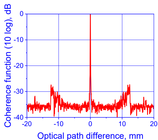
Coherence function
