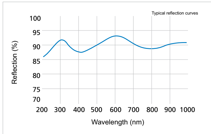
UV enhanced aluminum coating at 0°
