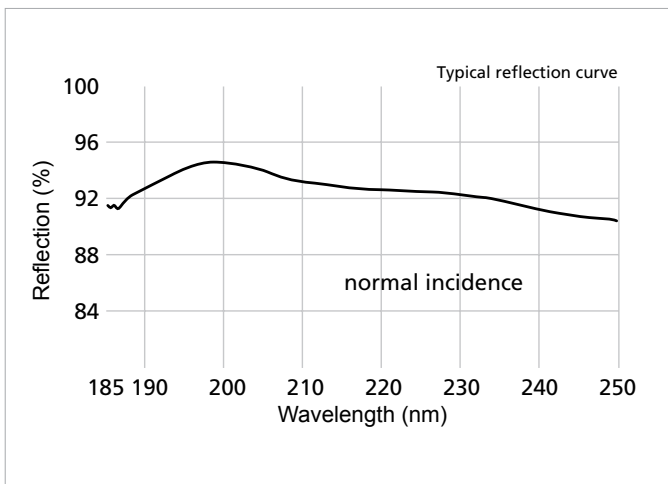
Reflection vs wavelength of 193nm deep UV aluminum coating at 0°
