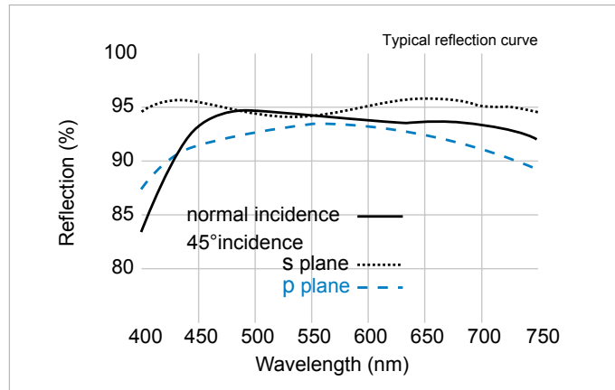
Enhanced aluminum coating
