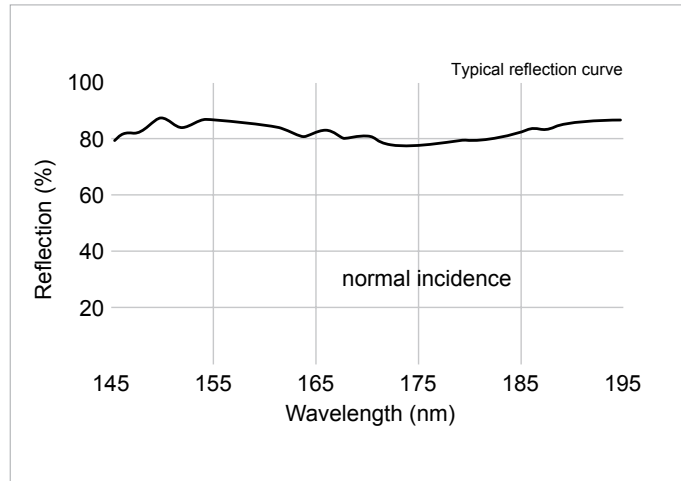
Theoretical design of VUVA coating at 157nm and 0°
