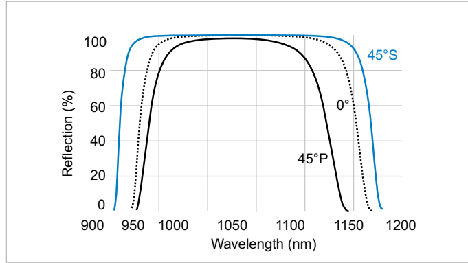
Reflectivity vs wavelength of FLM fiber laser mirror at 1030nm for 0° and 45° designs
