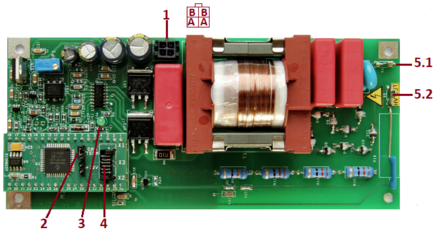
Figure 3. Top view of the HV power supply with CAN interface control (-C models)
