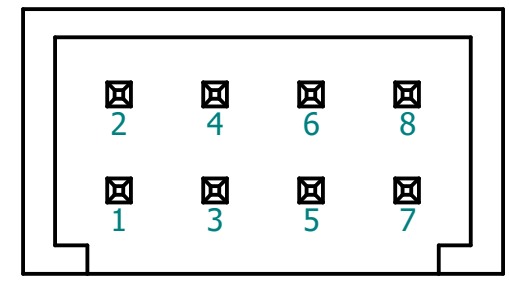
Power supply and TEC control socket AMPMODU 2x4 (male)
